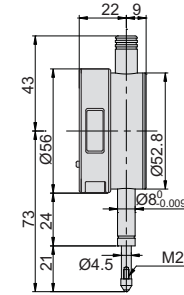
Range: 0-12.7mm
