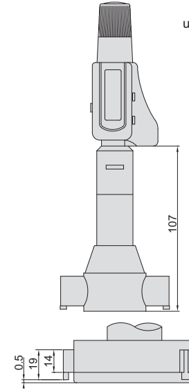
extension rod(included)
